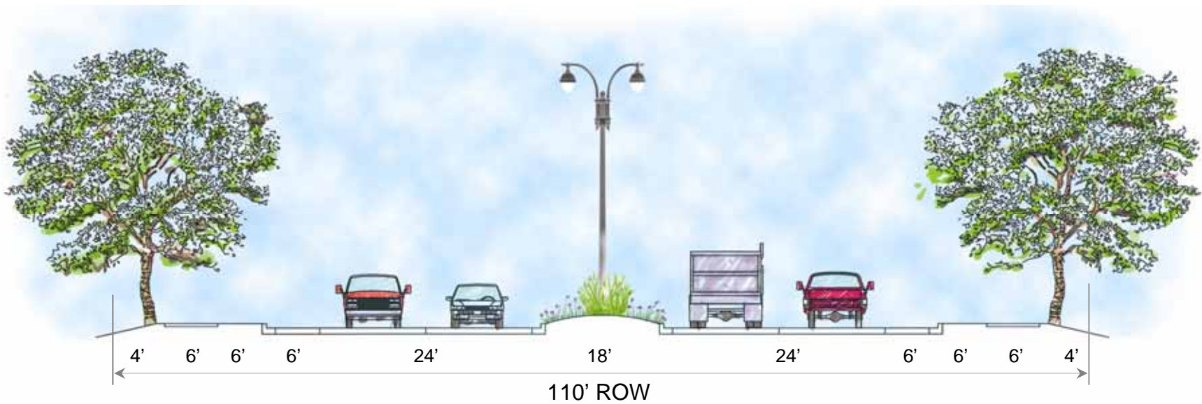
MSP Parkway Typical Section through Primary Road at Light Standard
