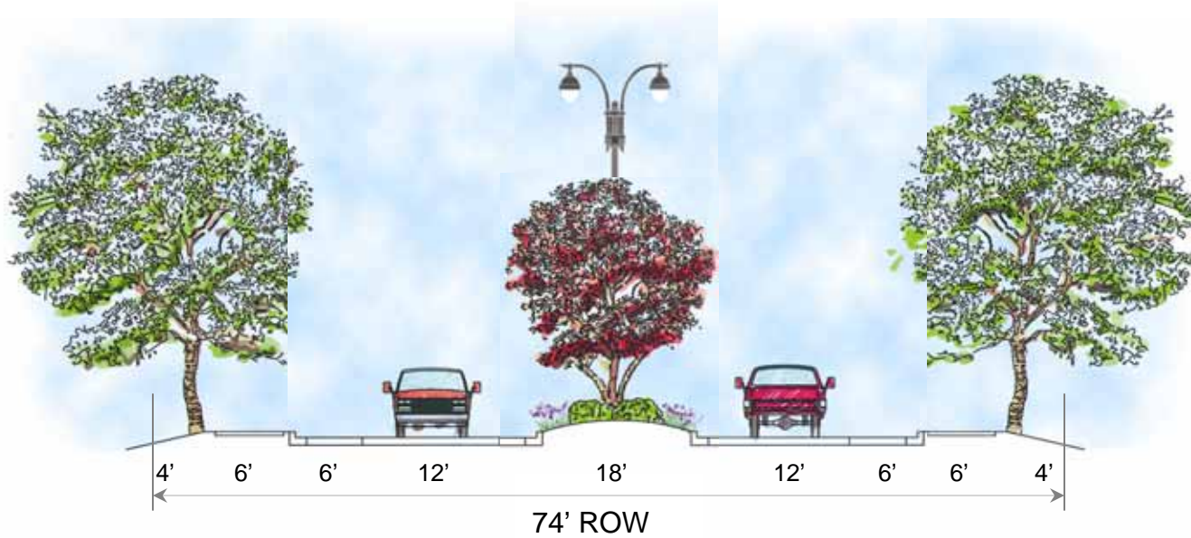
Typical Section through Chestnut Street and at Lafayette Street
