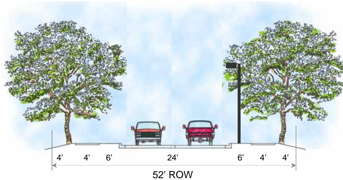
Typical Section through Tertiary Roadway
