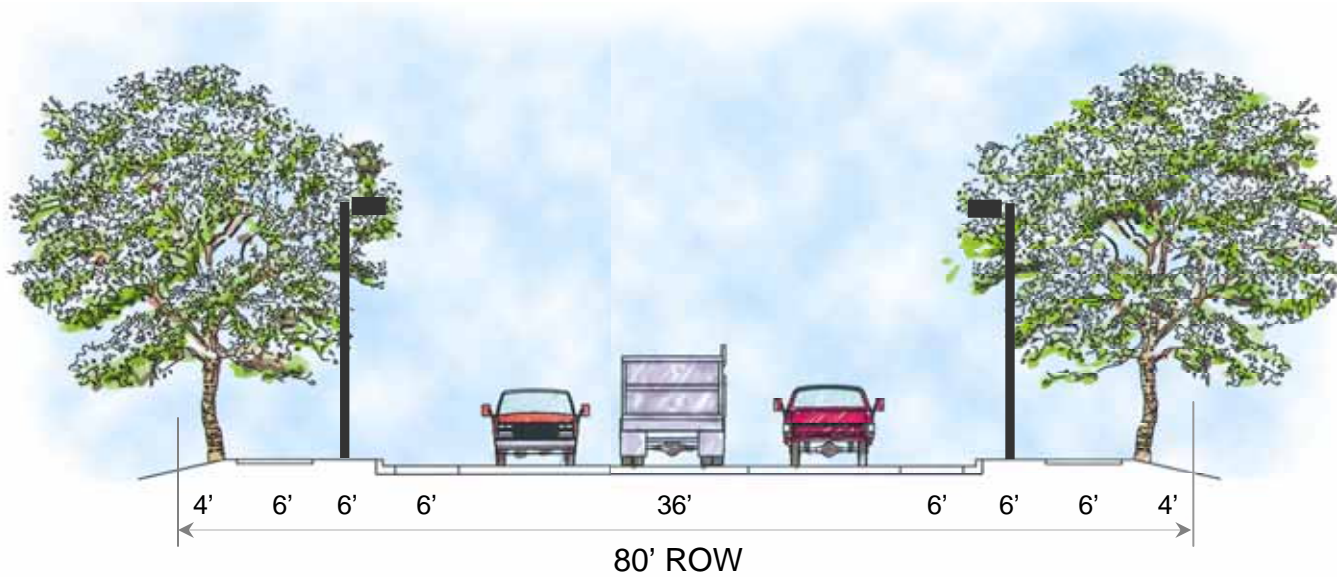
Typical Section through Secondary Roadway
