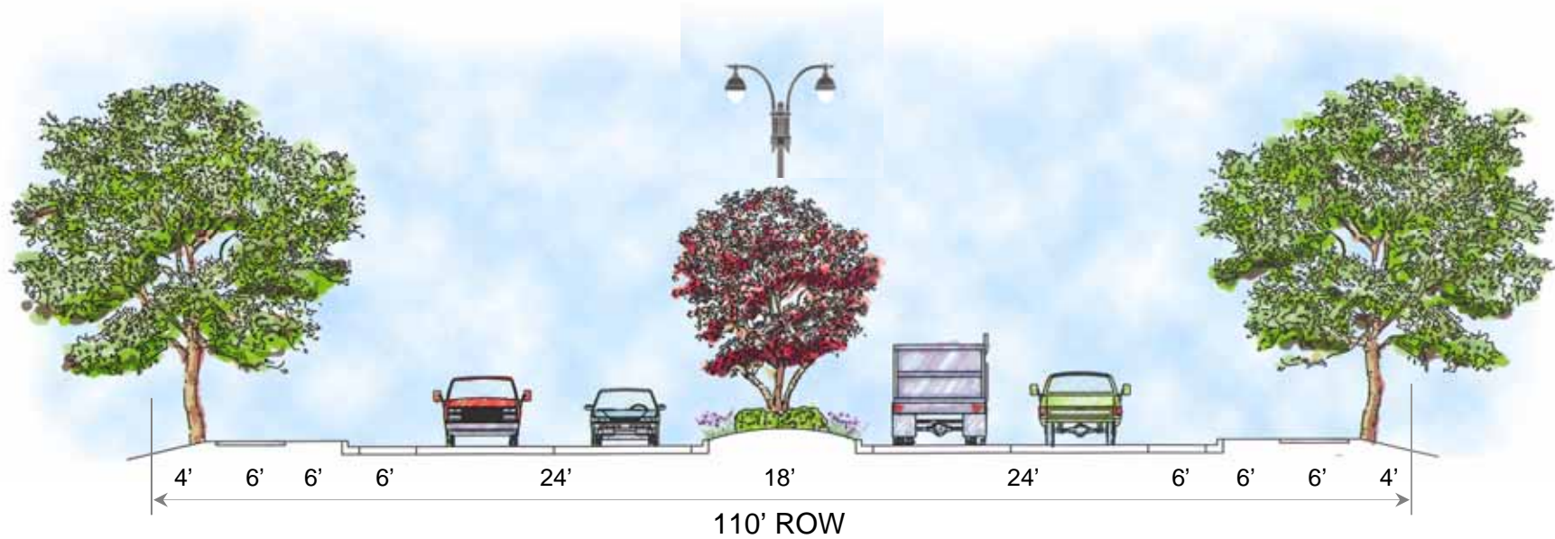
MSP Parkway Typical Section through Primary Road at Ornamental Trees
